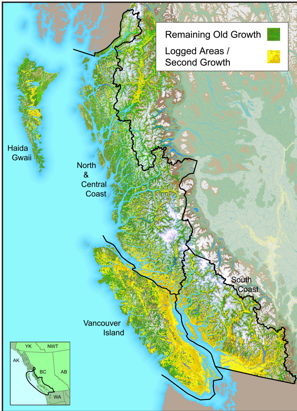
Map 1 – Remaining old growth rainforest and logged areas/second growth along British Columbia's Pacific Coast
